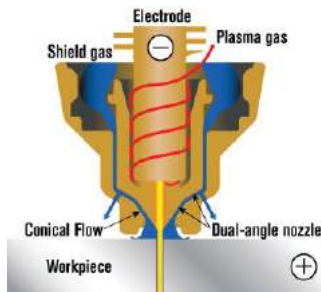
Conical Flow
